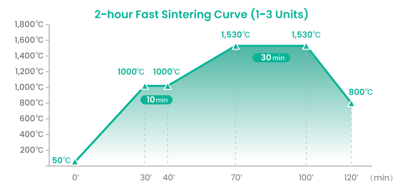
2-hour Fast Sintering Parameters (1-3 Units)
